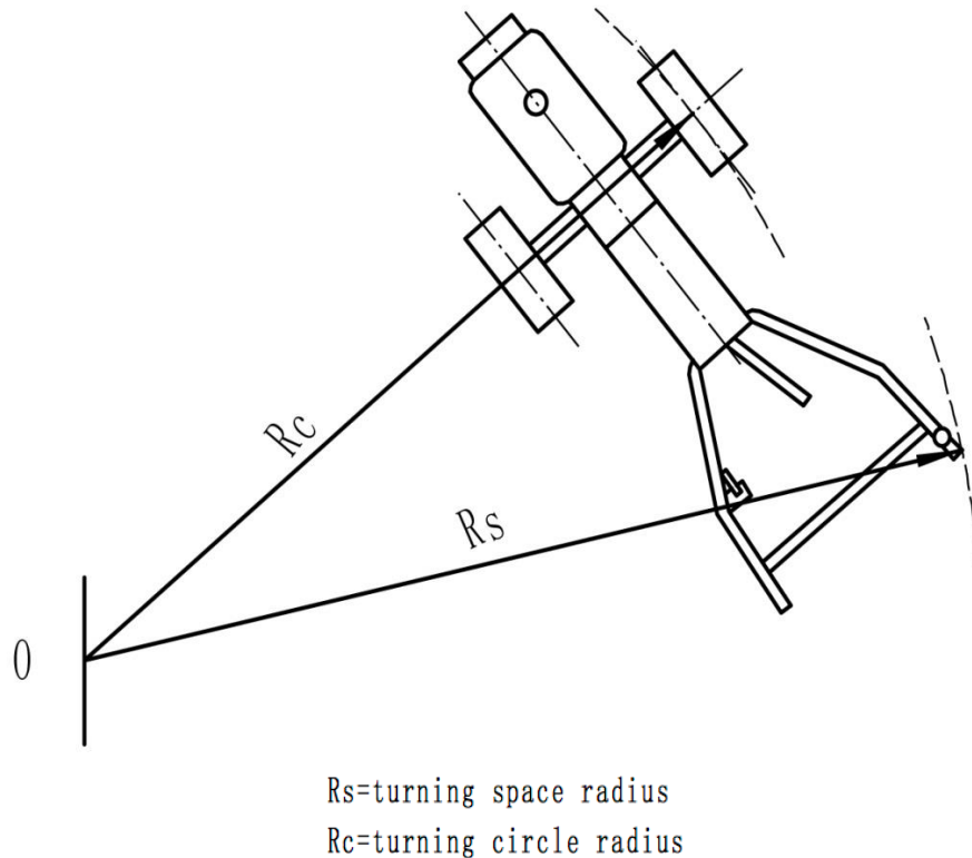
Figure 1: The measurement of radius of turning circle and turning space (6.3.1 GB/T 6229-2007)
